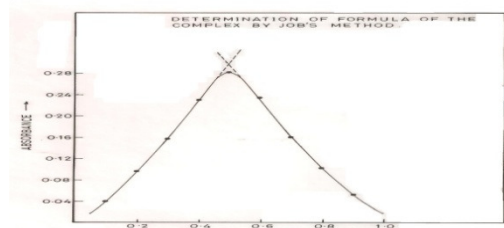
Figure 5: Job's method of continuous variation of F2STSC
