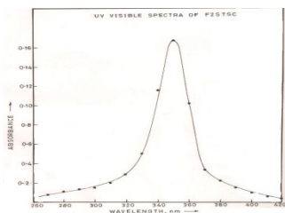
Figure 1: Absorption Spectra of F2STSC
