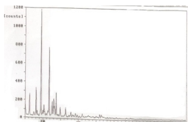
Figure 4: X-RD of F2STSC
