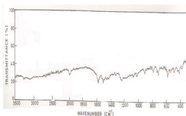
Figure 2: Infrared spectra of F2STSC
