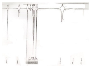
Figure 3: NMR spectra of F2STSC
